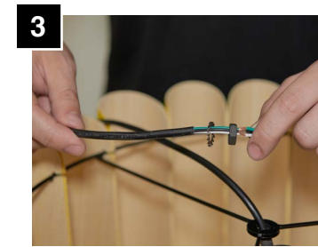
3 Pass lock washer and nut through cable.
